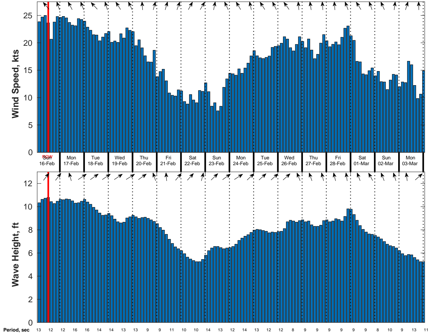
Wind & Wave Forecast for TOTAL Namibia GTS from 15-Feb-2025 02:00:00 to 03-Mar-2025 02:00:00
