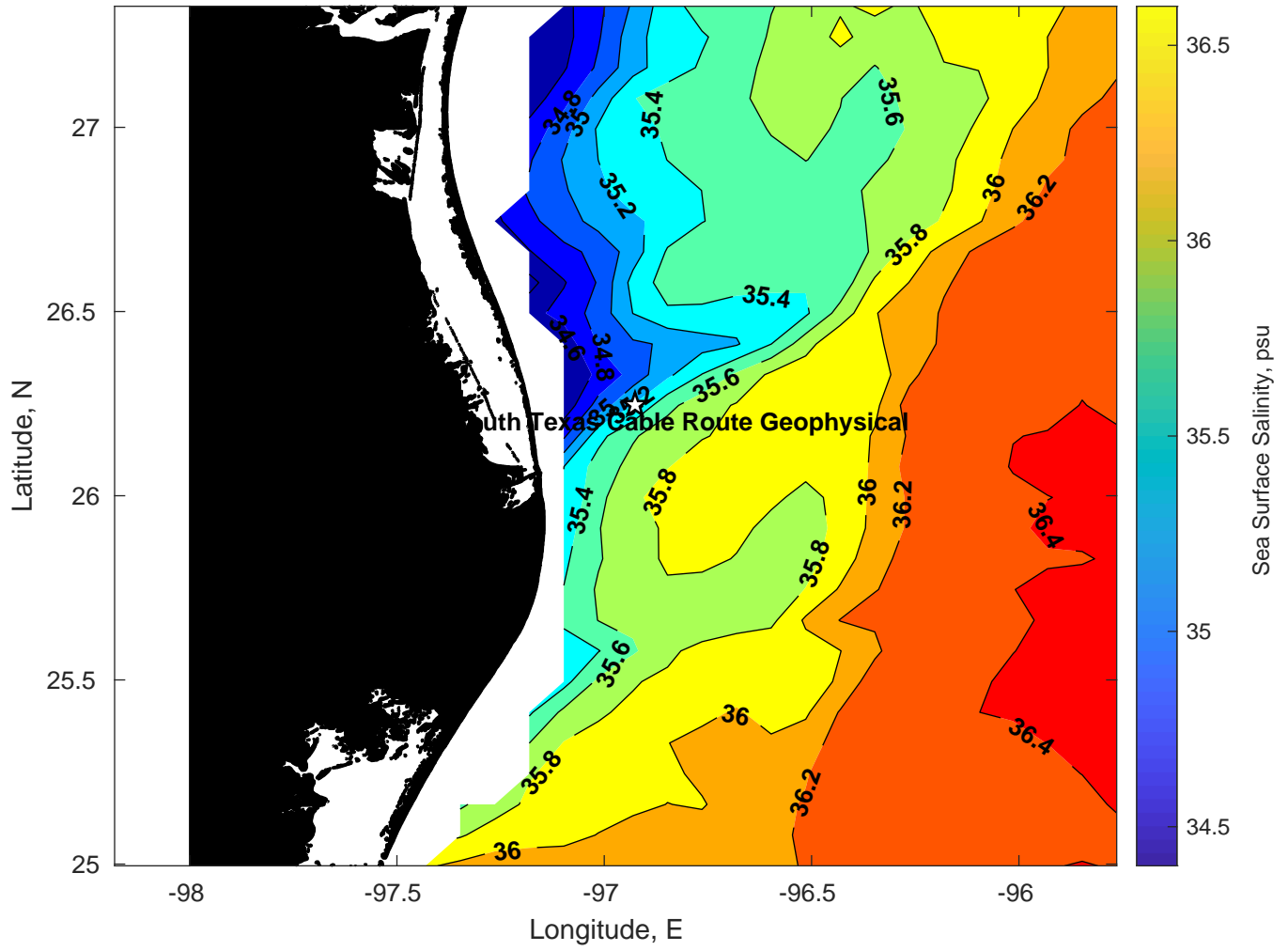
Surface Salinity for Tampnet P2378 South Texas Cable Route Geophysical at 14-Feb-2025 00:00:00
