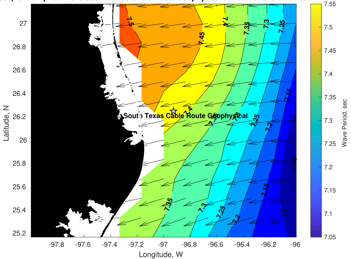
Period (sec) for Tampnet P2378 South Texas Cable Route Geophysical at 15-Feb-2025 09:00:00
