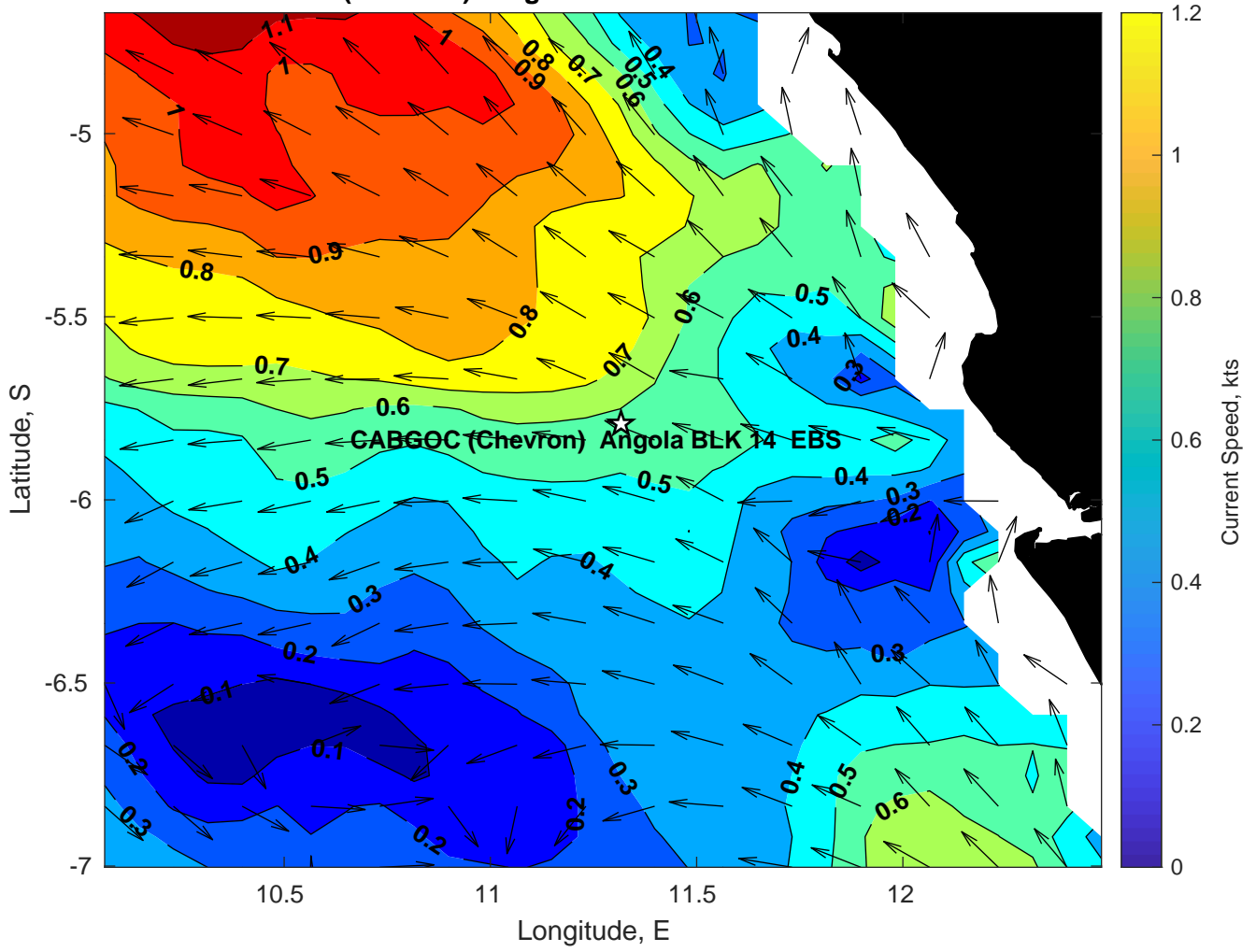
Surface Currents for CABGOC (Chevron) Angola BLK 14 EBS at 15-Feb-2025 00:00:00
