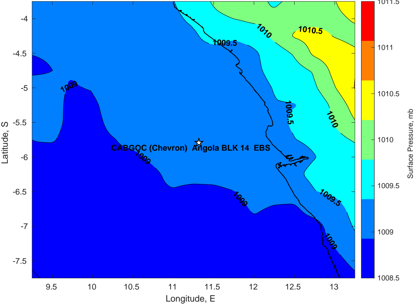
Surface Pressure (mb) for CABGOC (Chevron) Angola BLK 14 EBS at 18-Feb-2025 00:00:00
