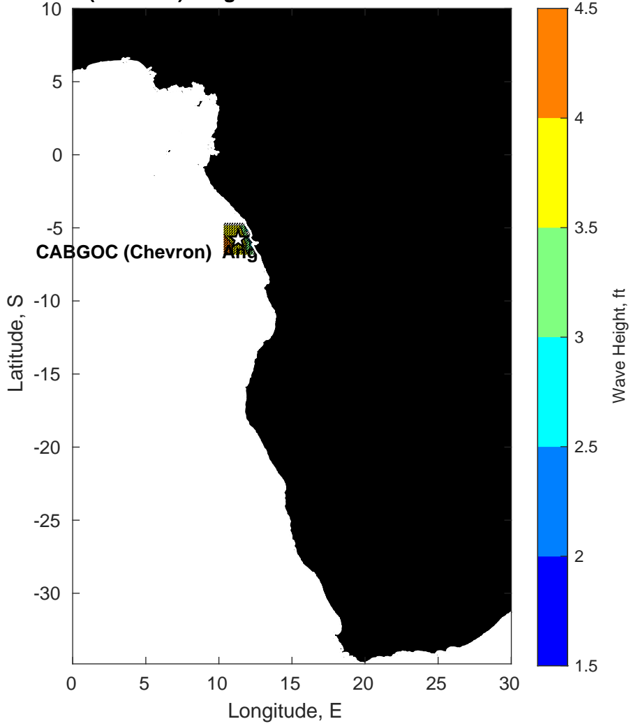
Wave Height (ft) for CABGOC (Chevron) Angola BLK 14 EBS at 16-Feb-2025 09:00:00
