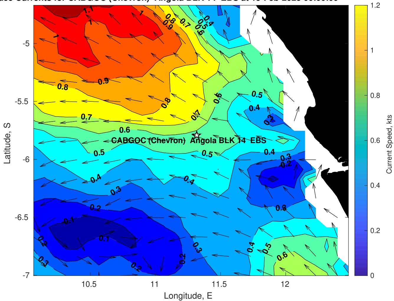
Surface Currents for CABGOC (Chevron) Angola BLK 14 EBS at 15-Feb-2025 00:00:00
