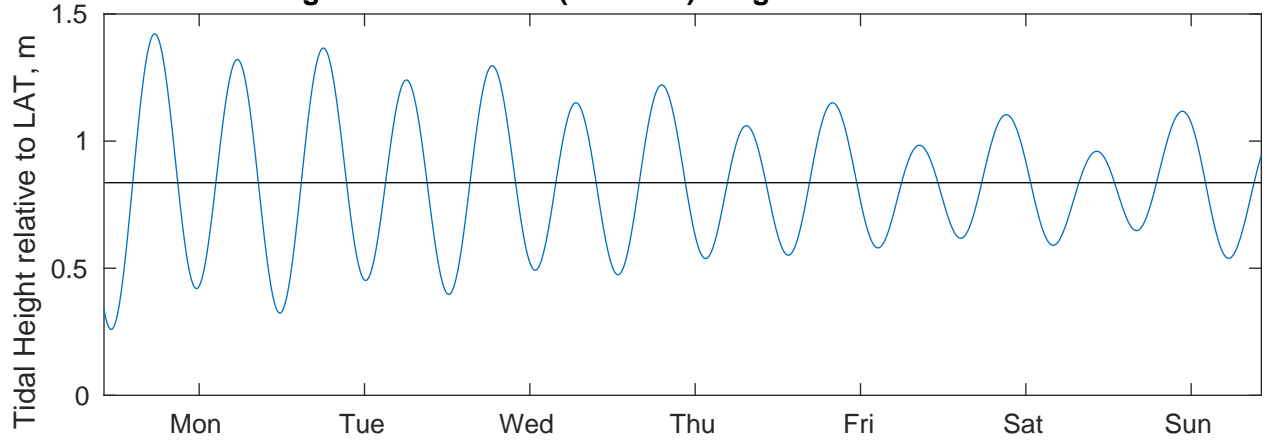
Tidal Currents and Heights for CABGOC (Chevron) Angola BLK 14 EBS at 20250216
