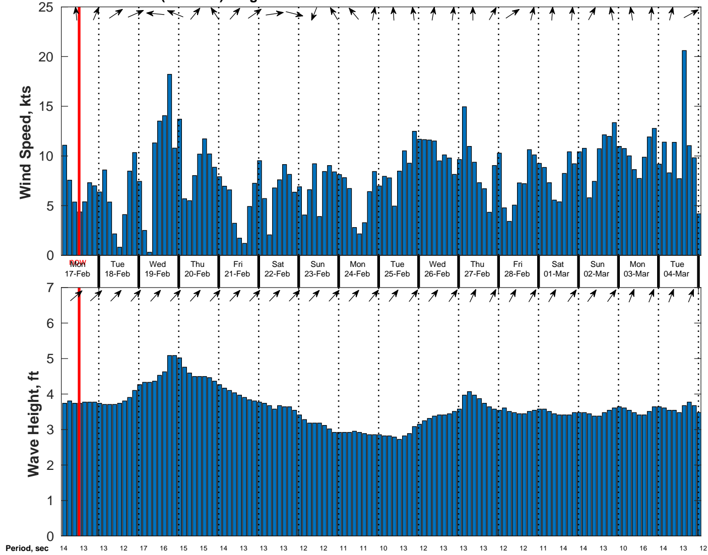
Wind & Wave Forecast for CABGOC (Chevron) Angola BLK 14 EBS from 16-Feb-2025 02:00:00 to 04-Mar-2025 02:00:00
