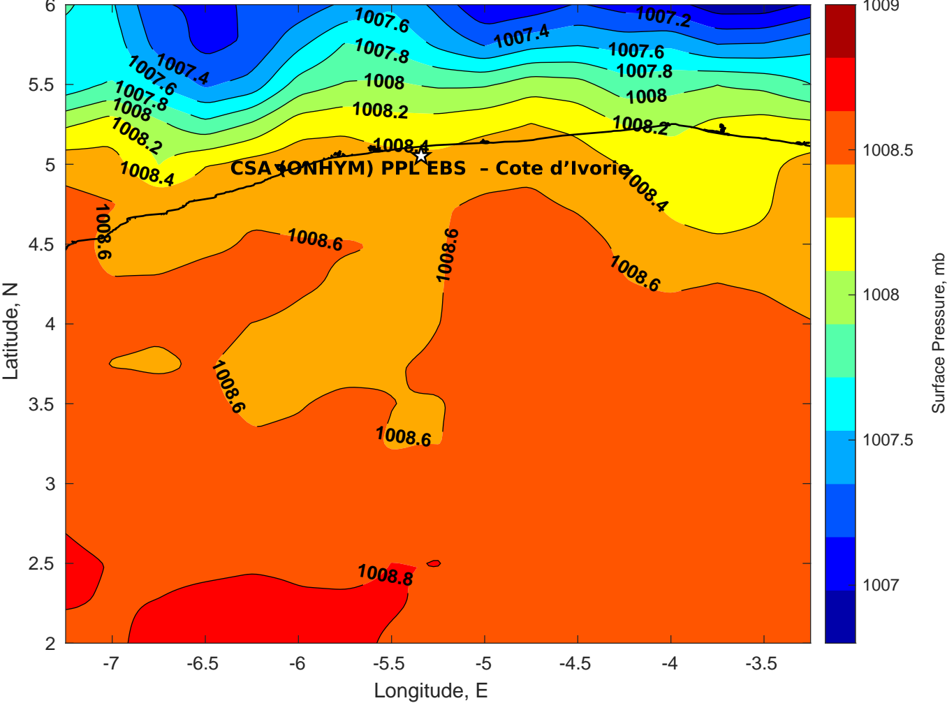
Surface Pressure (mb) for CSA (ONHYM) PPL EBS - Cote d'Ivoire at 16-Feb-2025 18:00:00
