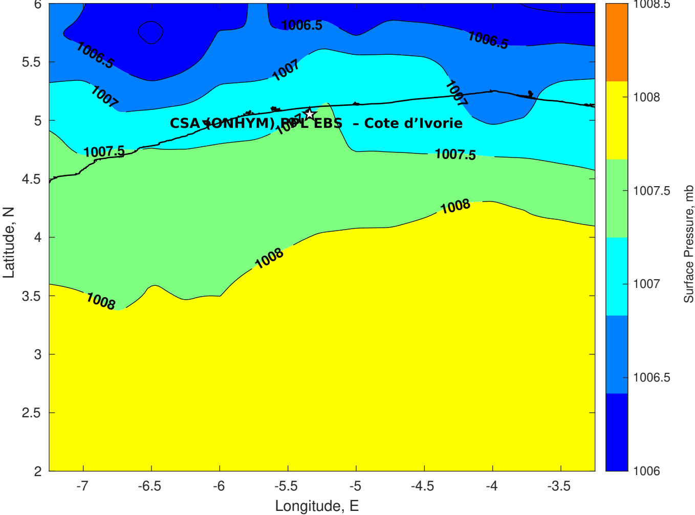
Surface Pressure (mb) for CSA (ONHYM) PPL EBS - Cote d'Ivoire at 17-Feb-2025 18:00:00
