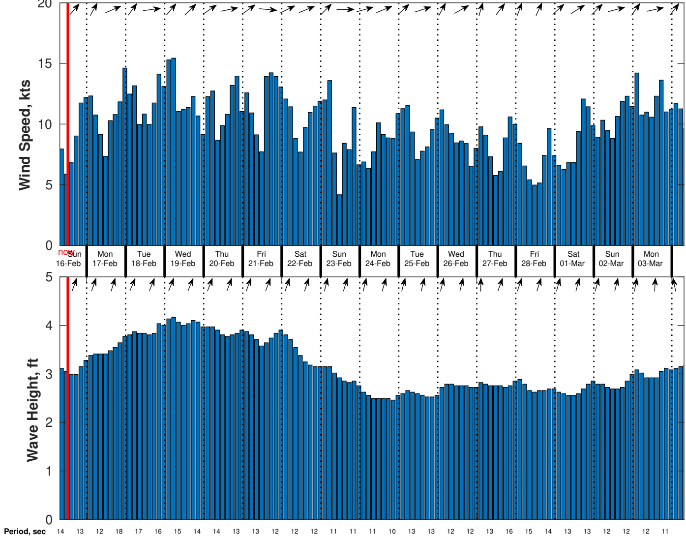
Wind & Wave Forecast for CSA (ONHYM) PPL EBS - Cote d'Ivoire from 16-Feb-2025 07:00:00 to 04-Mar-2025 07:00:00
