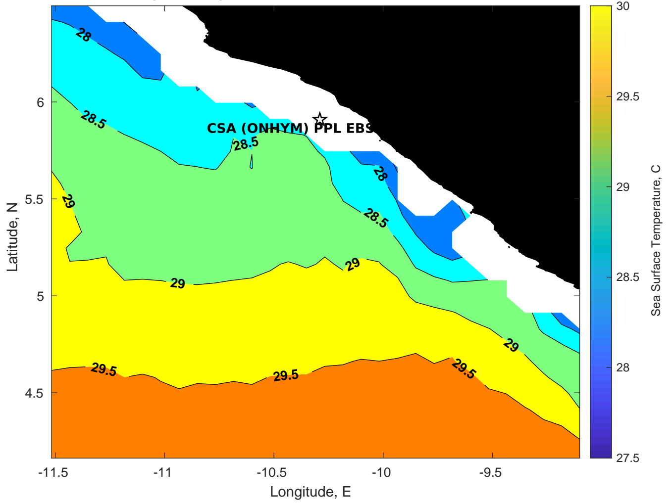
SST for CSA (ONHYM) PPL EBS - Liberia at 15-Feb-2025 00:00:00
