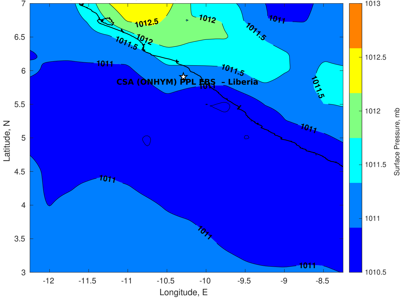
Surface Pressure (mb) for CSA (ONHYM) PPL EBS - Liberia at 16-Feb-2025 00:00:00
