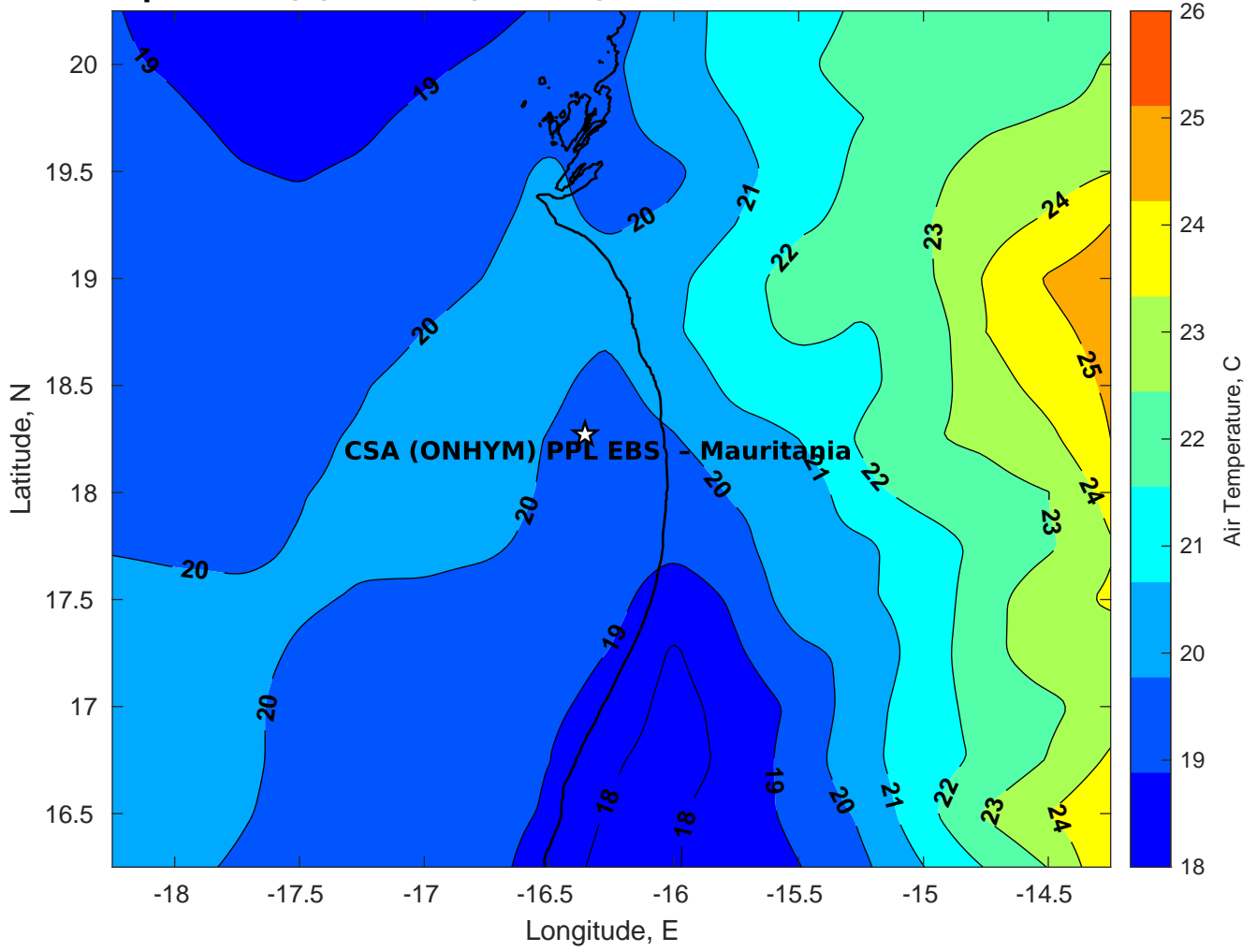
Air Temperature (C) for CSA (ONHYM) PPL EBS - Mauritania at 16-Feb-2025
