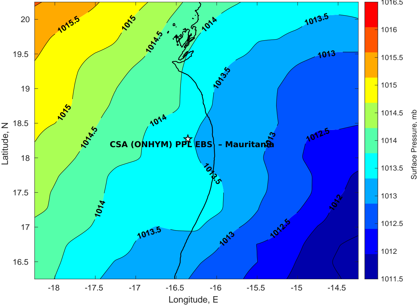
Surface Pressure (mb) for CSA (ONHYM) PPL EBS - Mauritania at 17-Feb-2025 00:00:00
