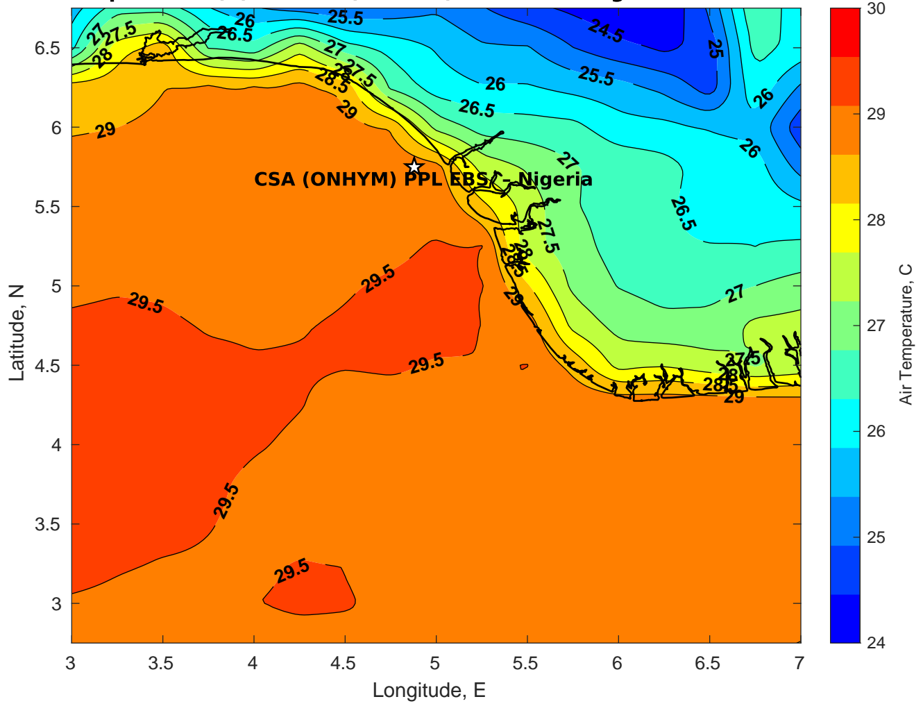
Air Temperature (C) for CSA (ONHYM) PPL EBS - Nigeria at 16-Feb-2025
