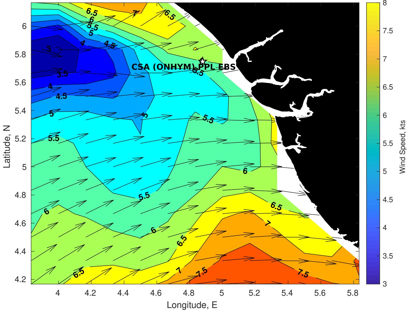
Winds (kts) for CSA (ONHYM) PPL EBS - Nigeria at 16-Feb-2025 09:00:00
