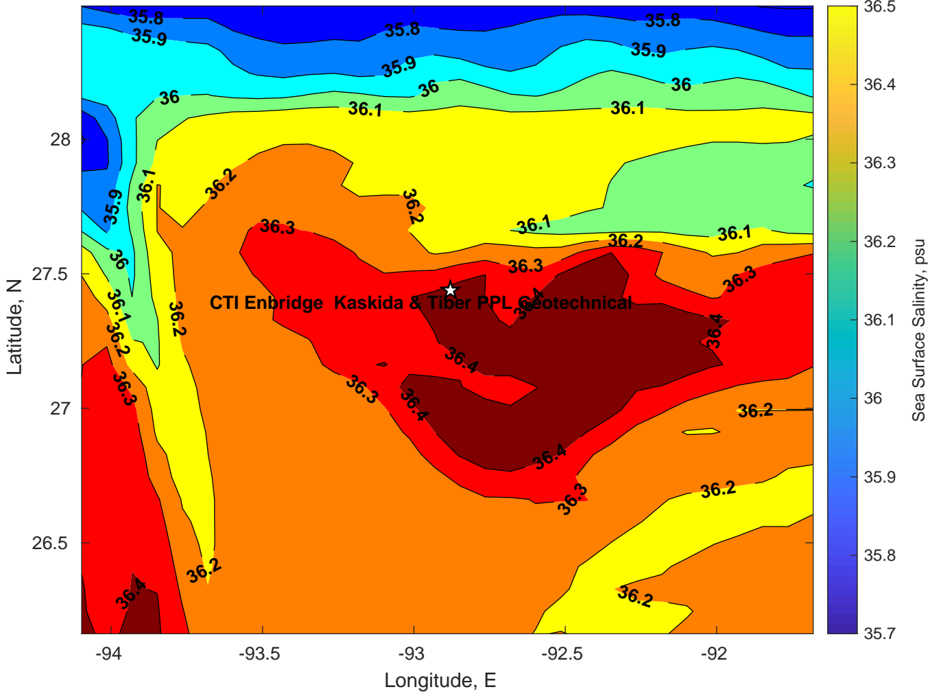
Surface Salinity for CTI Enbridge Kaskida & Tiber PPL Geotechnical at 15-Feb-2025 00:00:00
