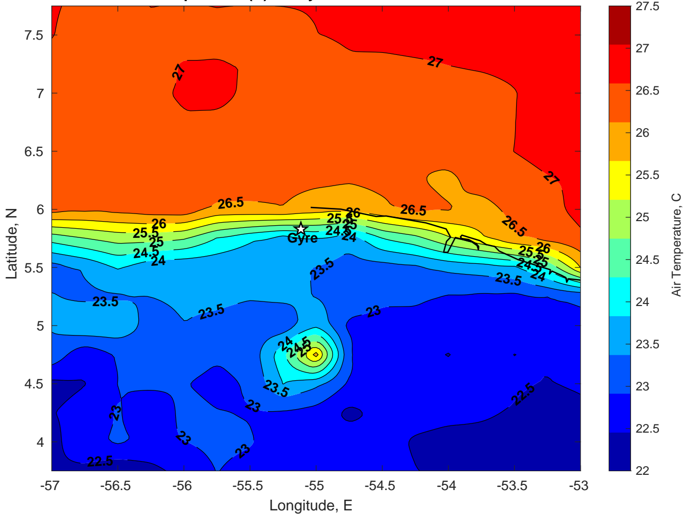
Air Temperature (C) for Gyre at 16-Feb-2025
