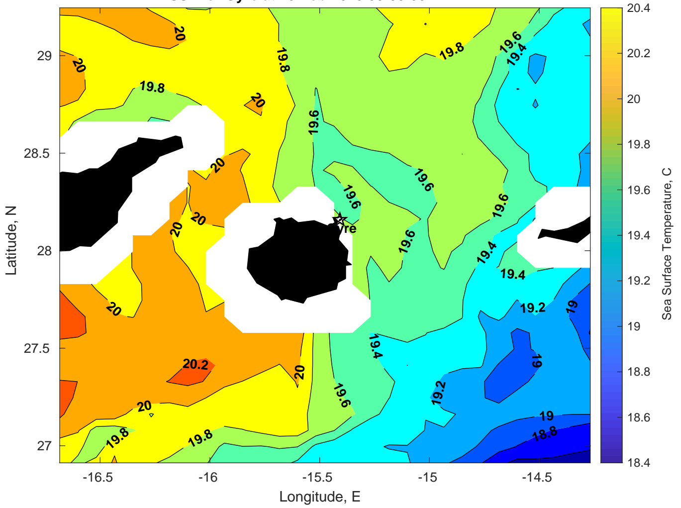
SST for Gyre at 15-Feb-2025 00:00:00
