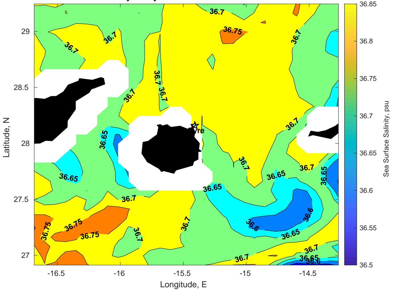
Surface Salinity for Gyre at 15-Feb-2025 00:00:00
