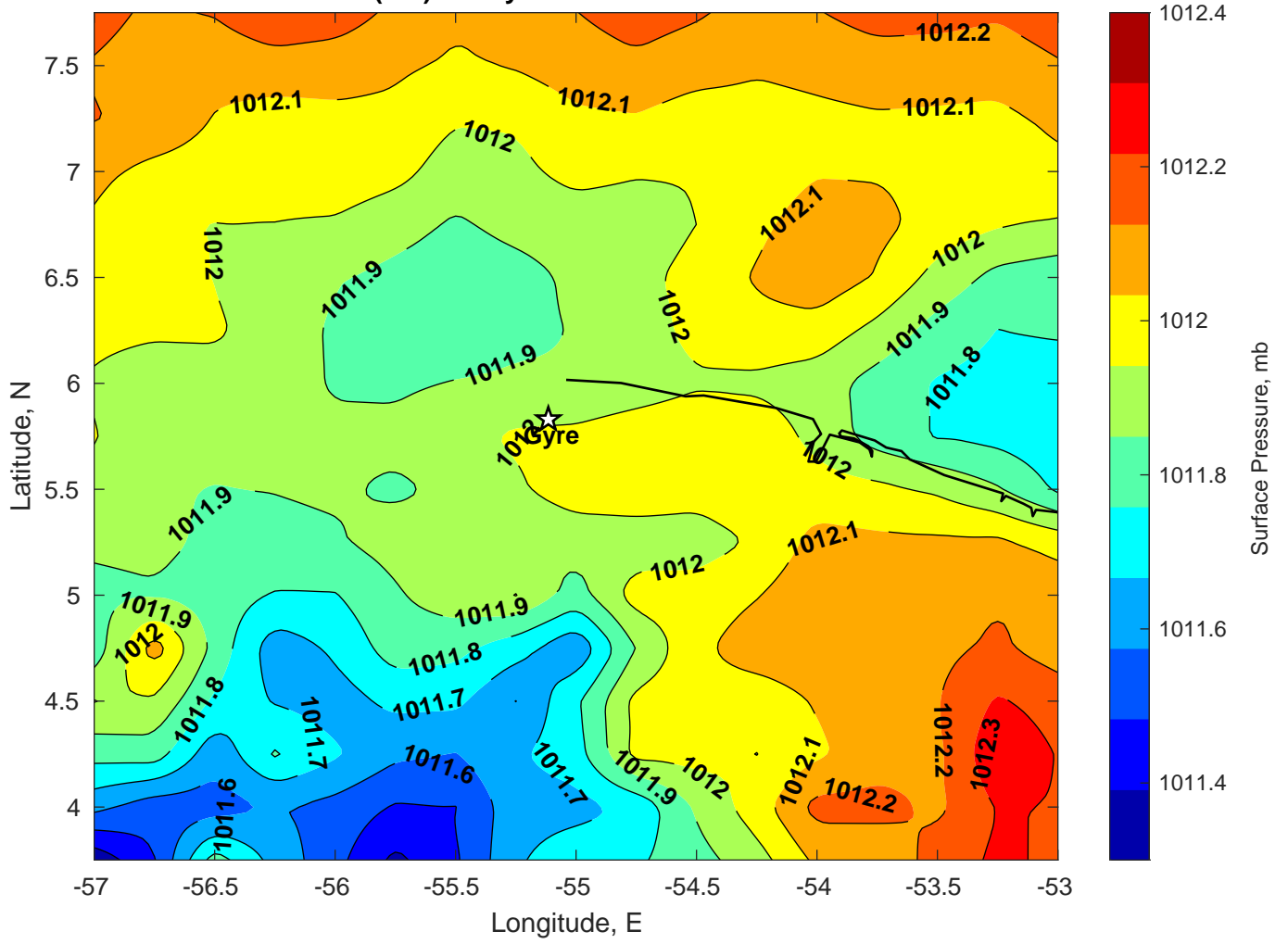
Surface Pressure (mb) for Gyre at 16-Feb-2025 00:00:00
