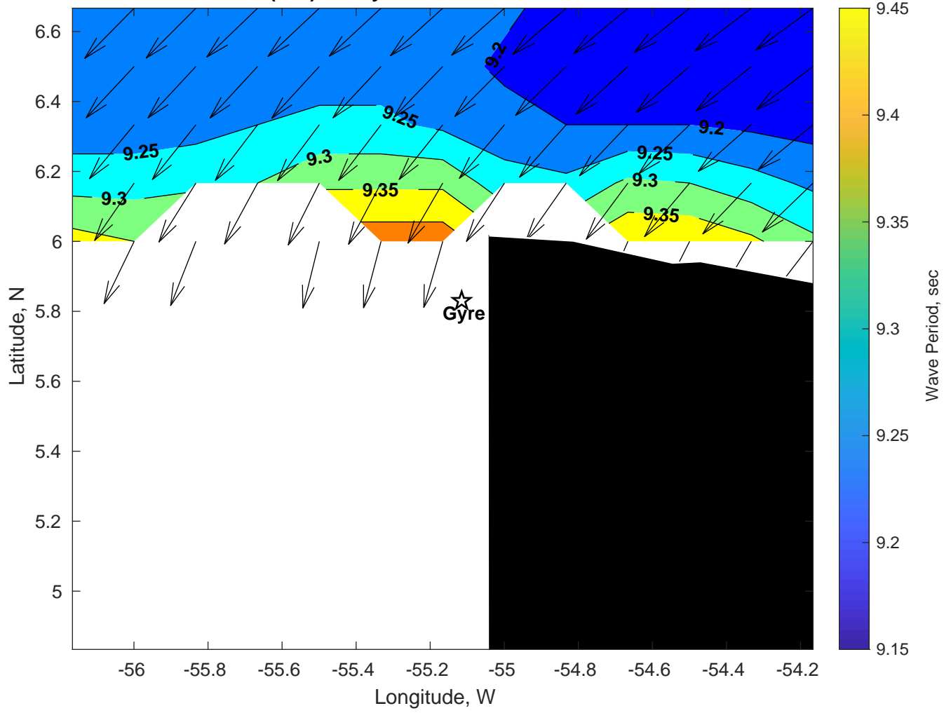
Wave Period (sec) for Gyre at 16-Feb-2025 09:00:00
