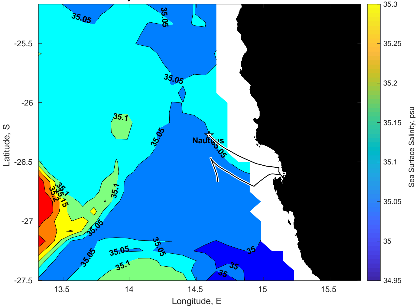
Surface Salinity for Nautilus at 15-Feb-2025 00:00:00
