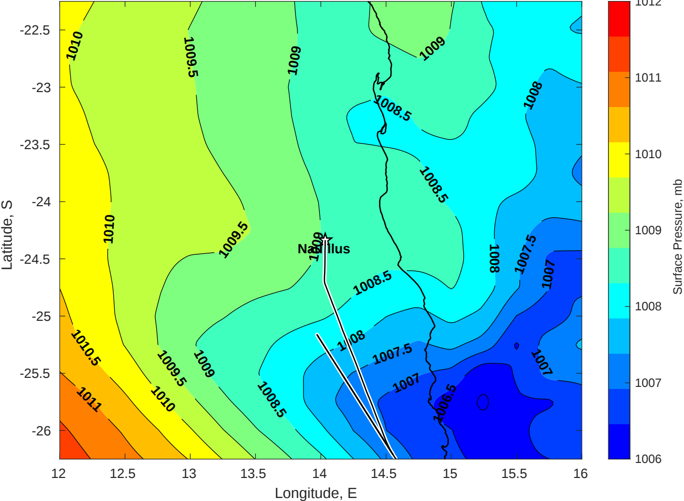
Surface Pressure (mb) for Nautilus at 17-Feb-2025 00:00:00
