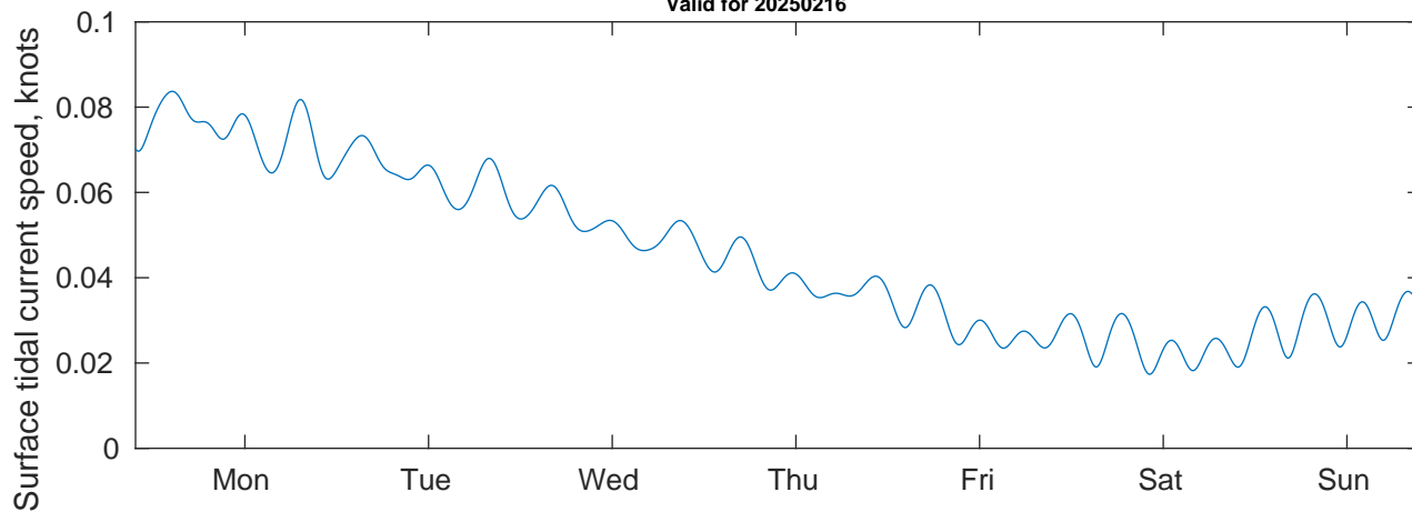
Tidal Currents and Heights for Nautilus at 20250216
