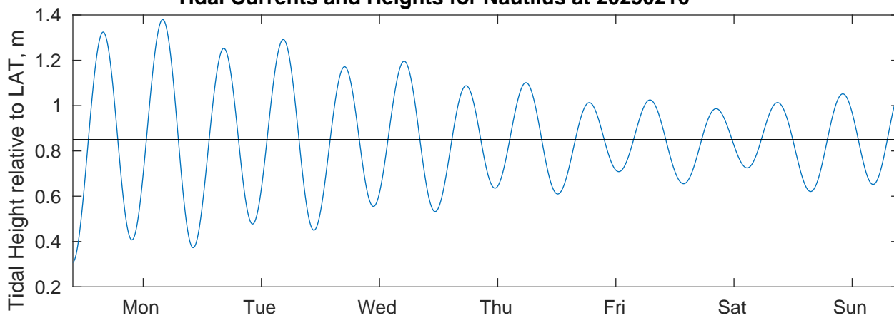
Tidal Currents and Heights for Nautilus at 20250216
