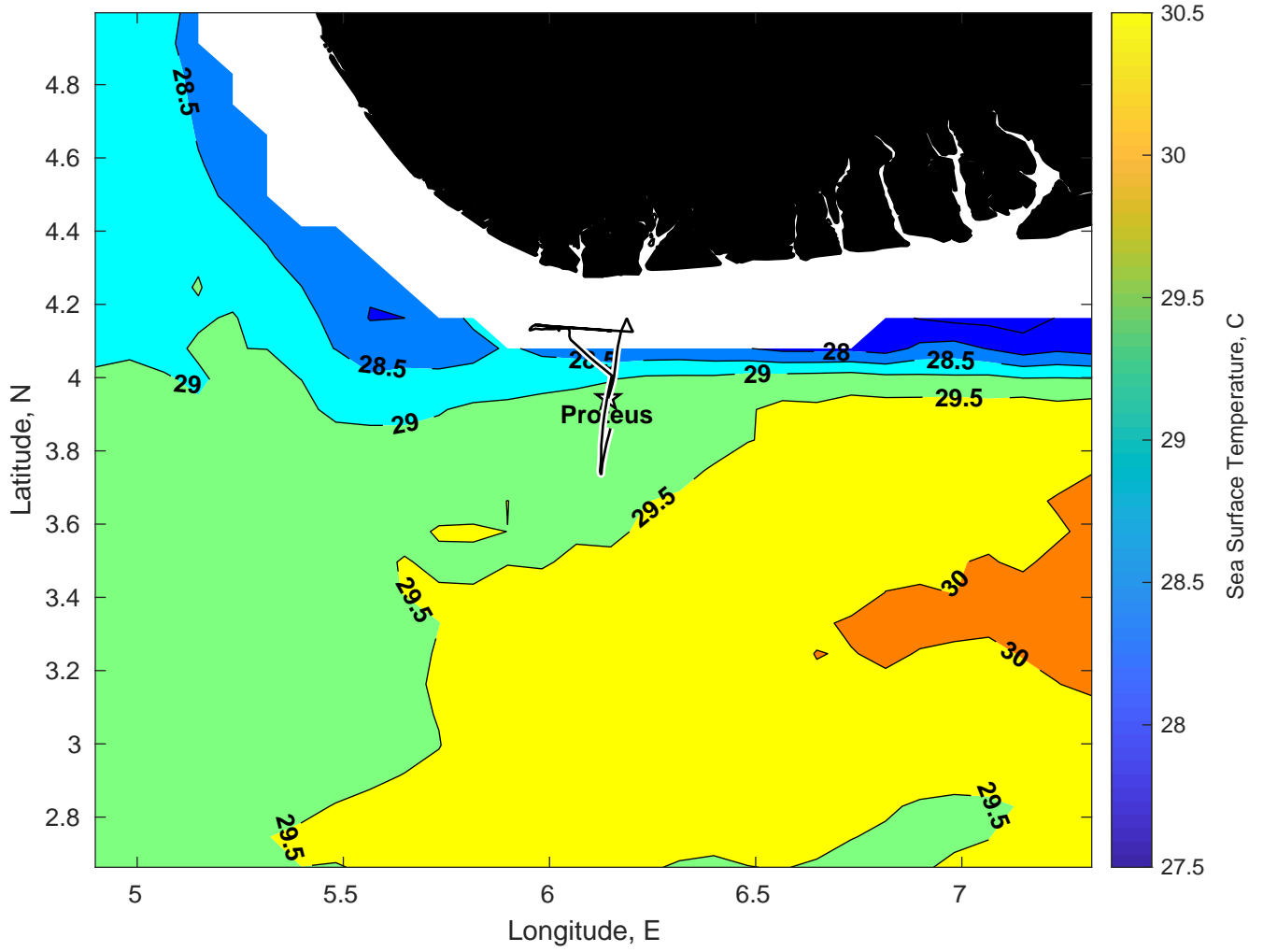
SST for Proteus at 15-Feb-2025 00:00:00
