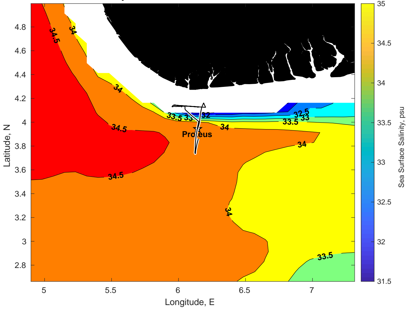
Surface Salinity for Proteus at 15-Feb-2025 00:00:00
