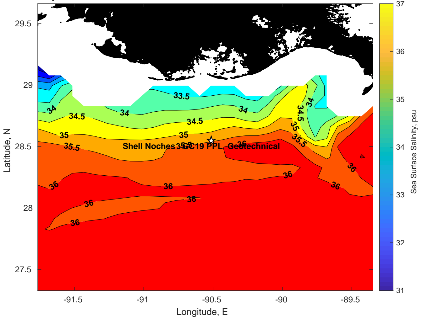
Surface Salinity for Shell Noches GC19 PPL Geotechnical at 15-Feb-2025 00:00:00
