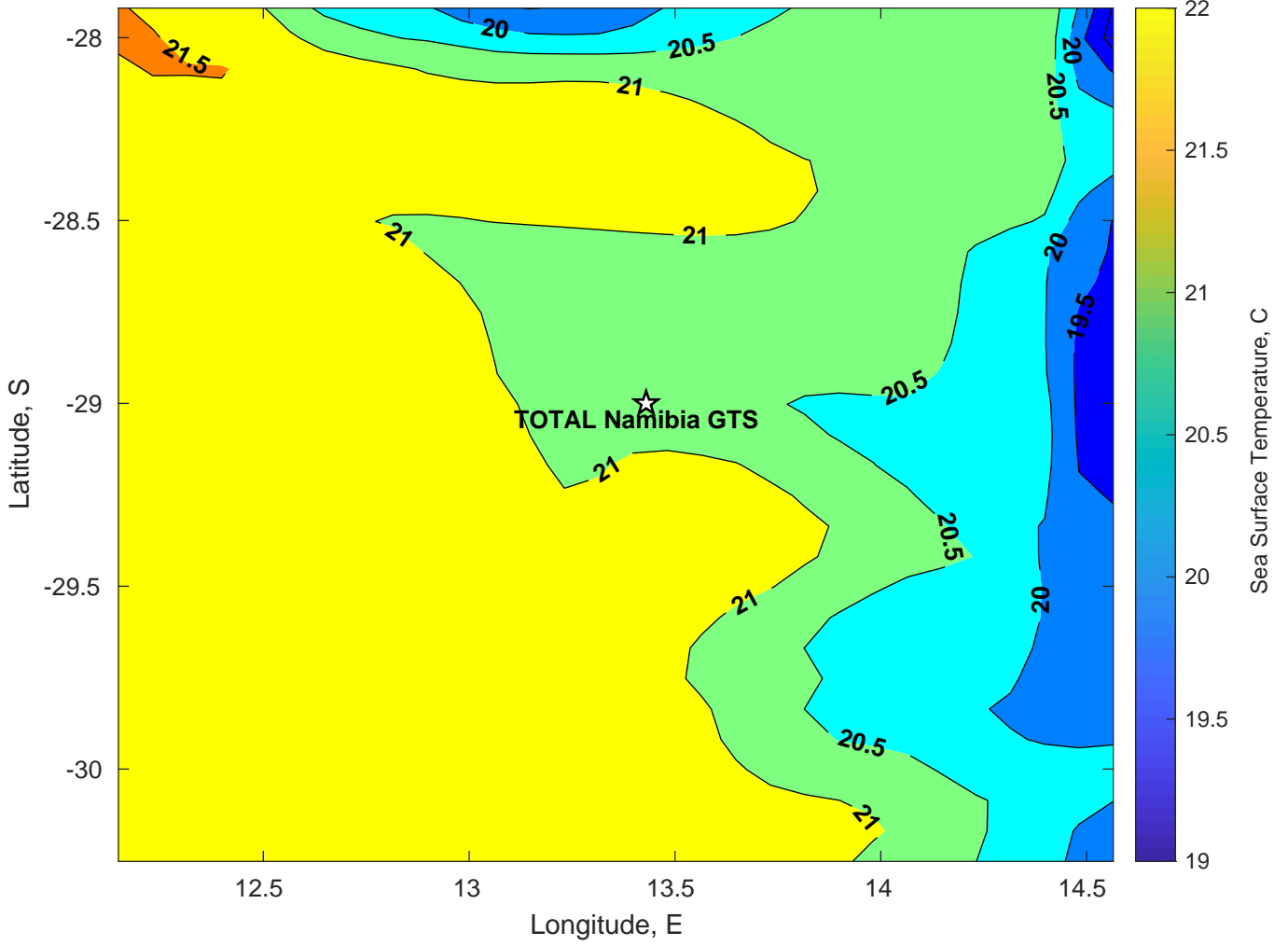
SST for TOTAL Namibia GTS at 15-Feb-2025 00:00:00
