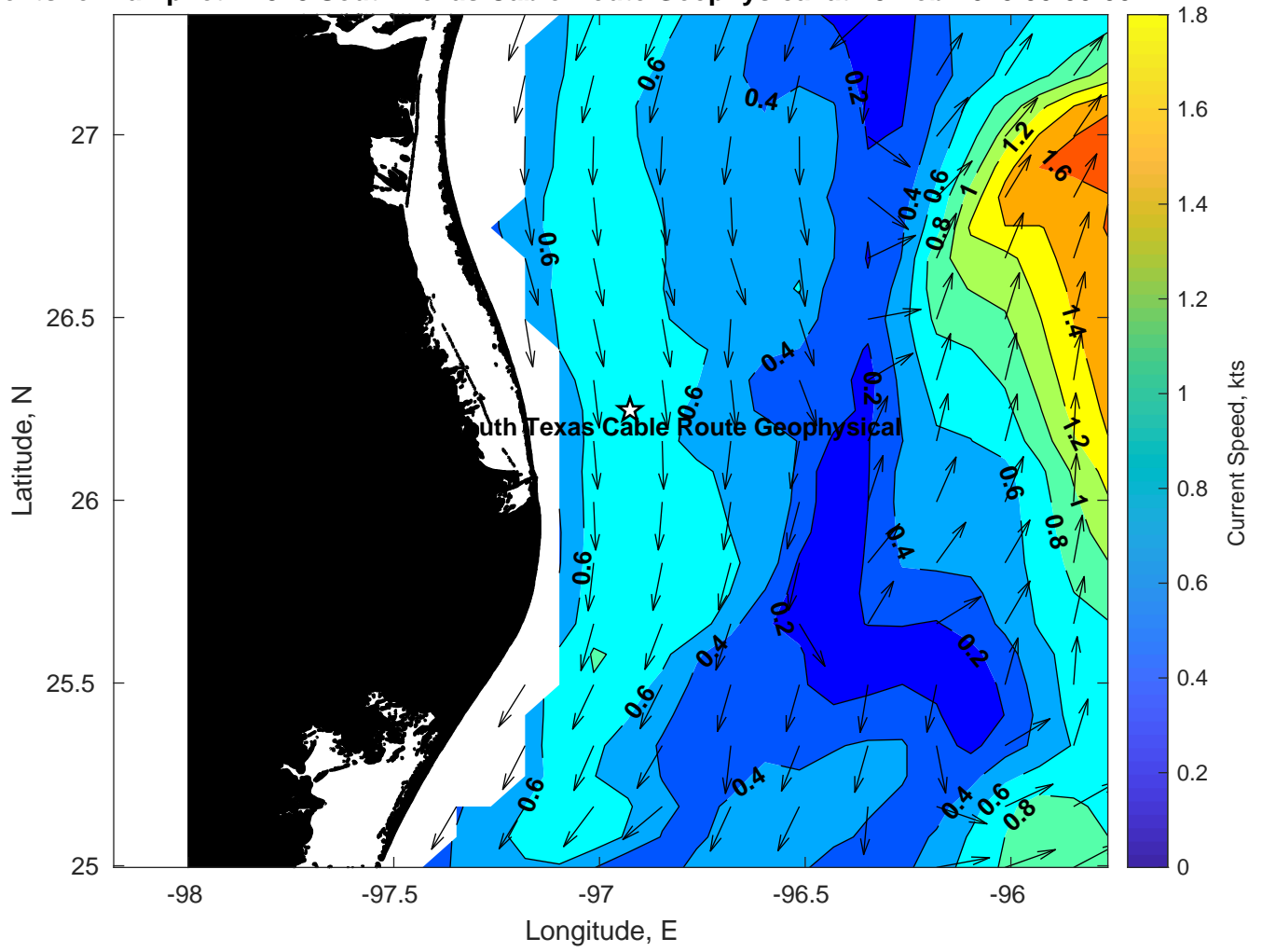
Surface Currents for Tampnet P2378 South Texas Cable Route Geophysical at 15-Feb-2025 00:00:00
