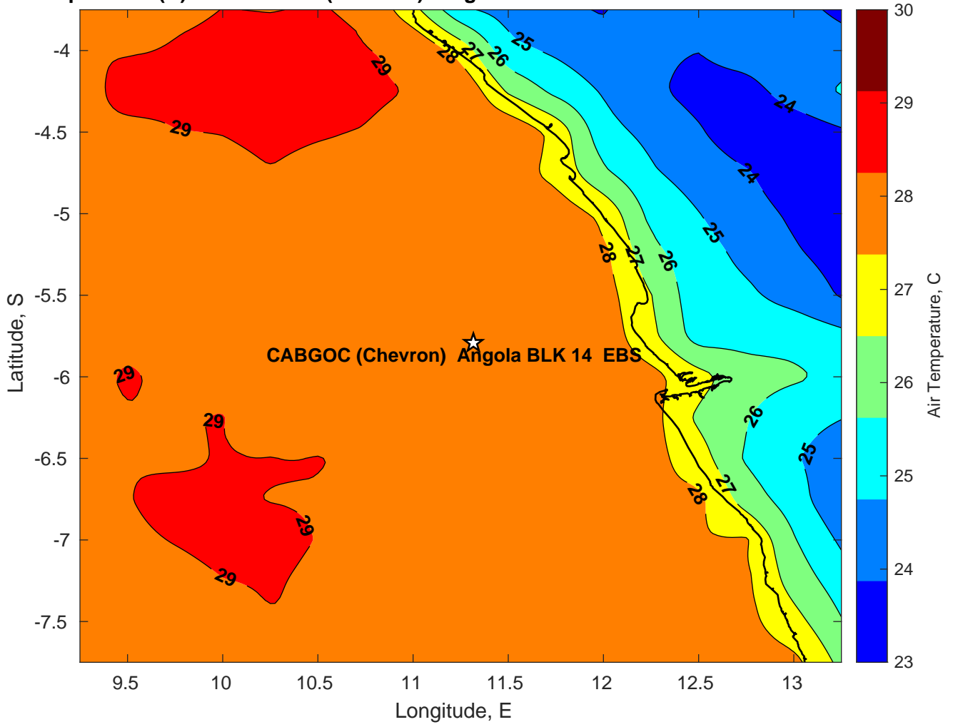
Air Temperature (C) for CABGOC (Chevron) Angola BLK 14 EBS at 17-Feb-2025
