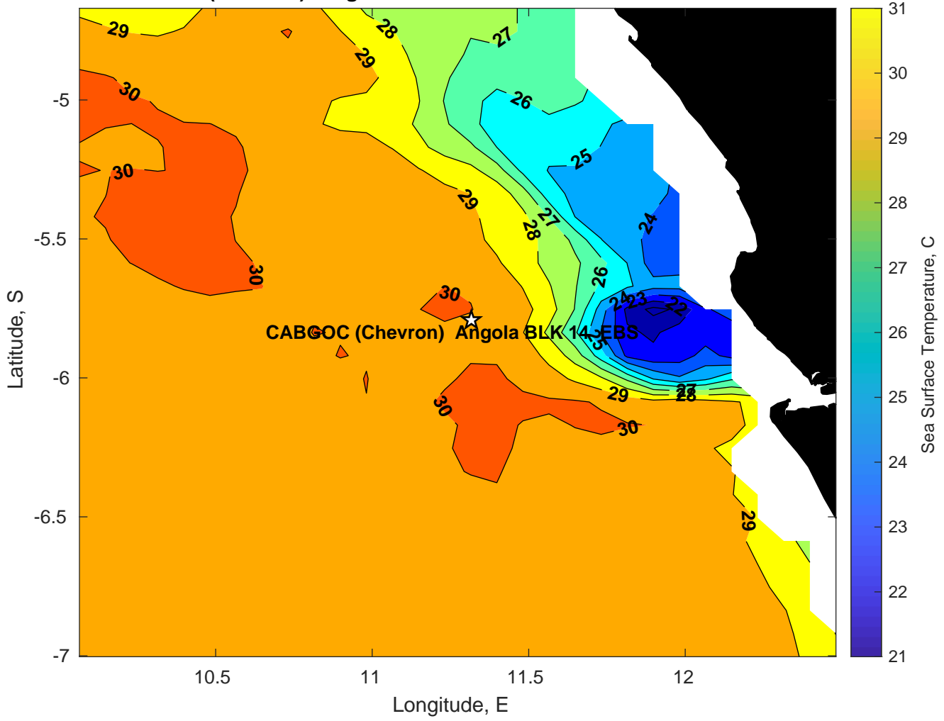
SST for CABGOC (Chevron) Angola BLK 14 EBS at 16-Feb-2025 00:00:00
