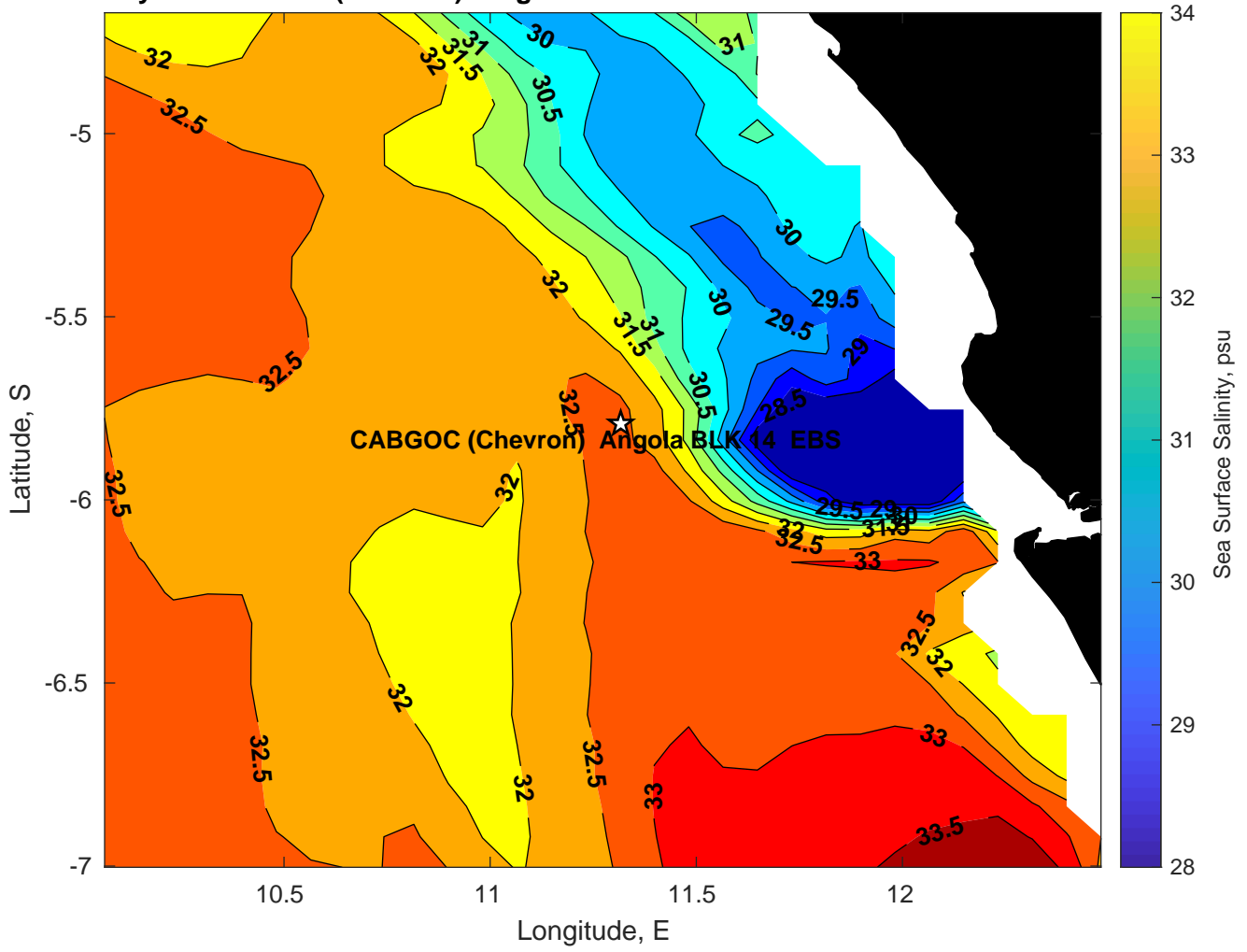
Surface Salinity for CABGOC (Chevron) Angola BLK 14 EBS at 16-Feb-2025 00:00:00
