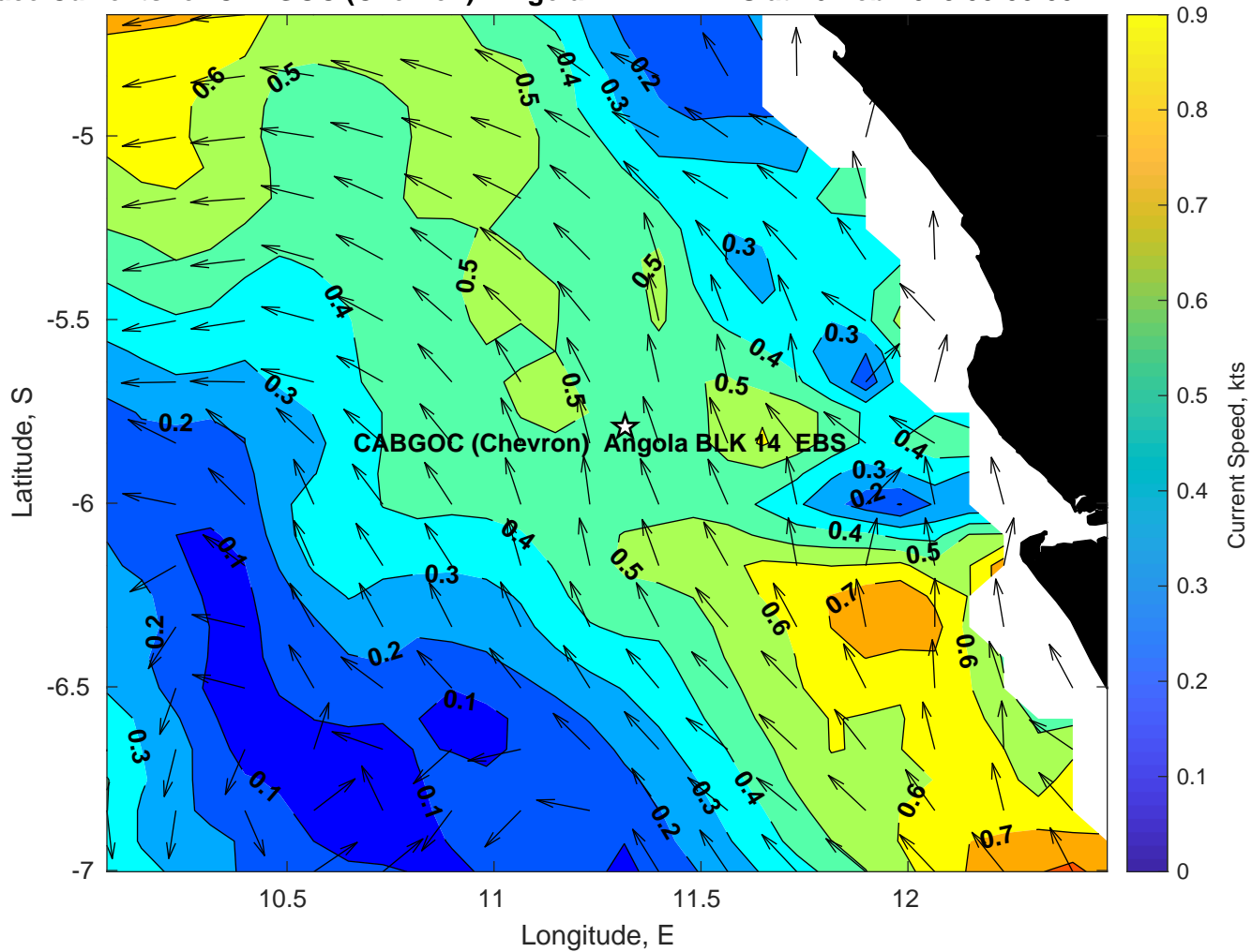
Surface Currents for CABGOC (Chevron) Angola BLK 14 EBS at 16-Feb-2025 00:00:00
