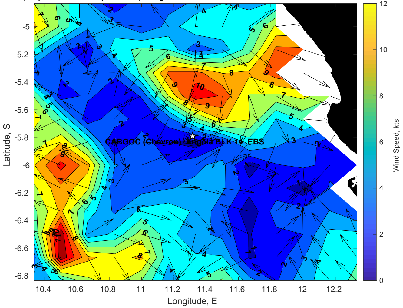
Winds (kts) for CABGOC (Chevron) Angola BLK 14 EBS at 17-Feb-2025 09:00:00
