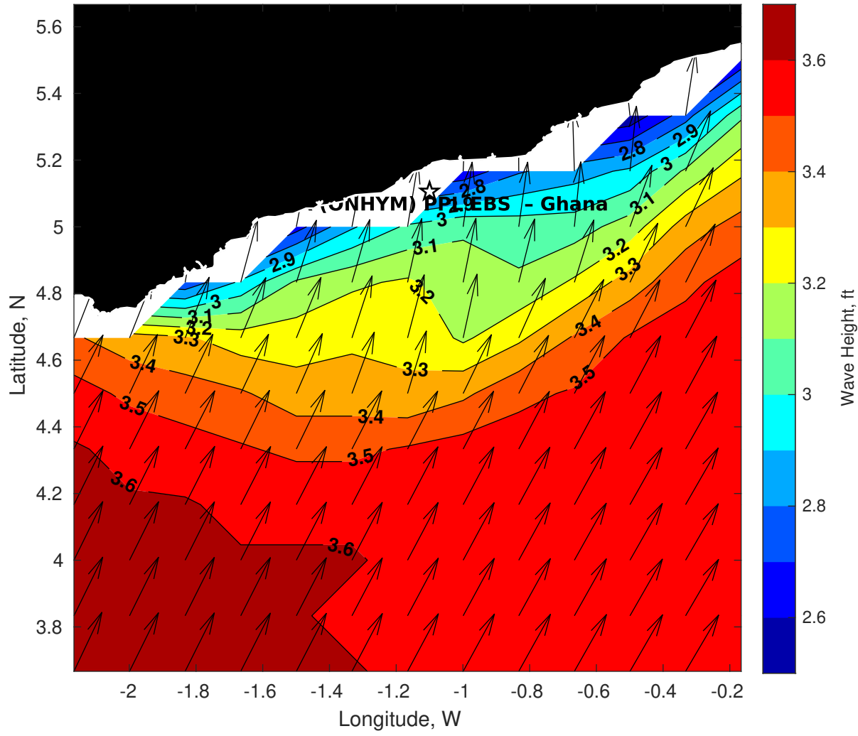
Wave Height (ft) for CSA (ONHYM) PPL EBS - Ghana at 17-Feb-2025 09:00:00
