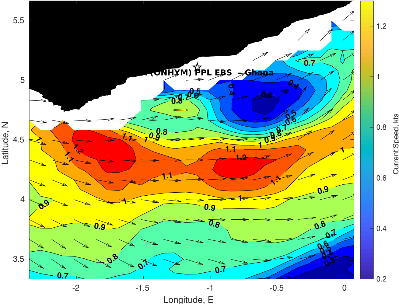
Surface Currents for CSA (ONHYM) PPL EBS - Ghana at 16-Feb-2025 00:00:00
