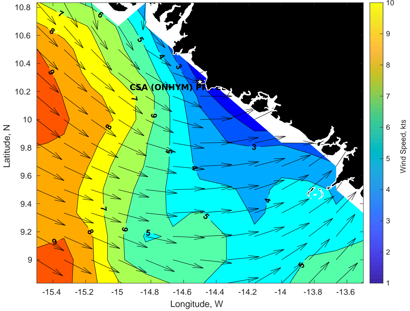
Winds (kts) for CSA (ONHYM) PPL EBS - Guinea at 17-Feb-2025 09:00:00
