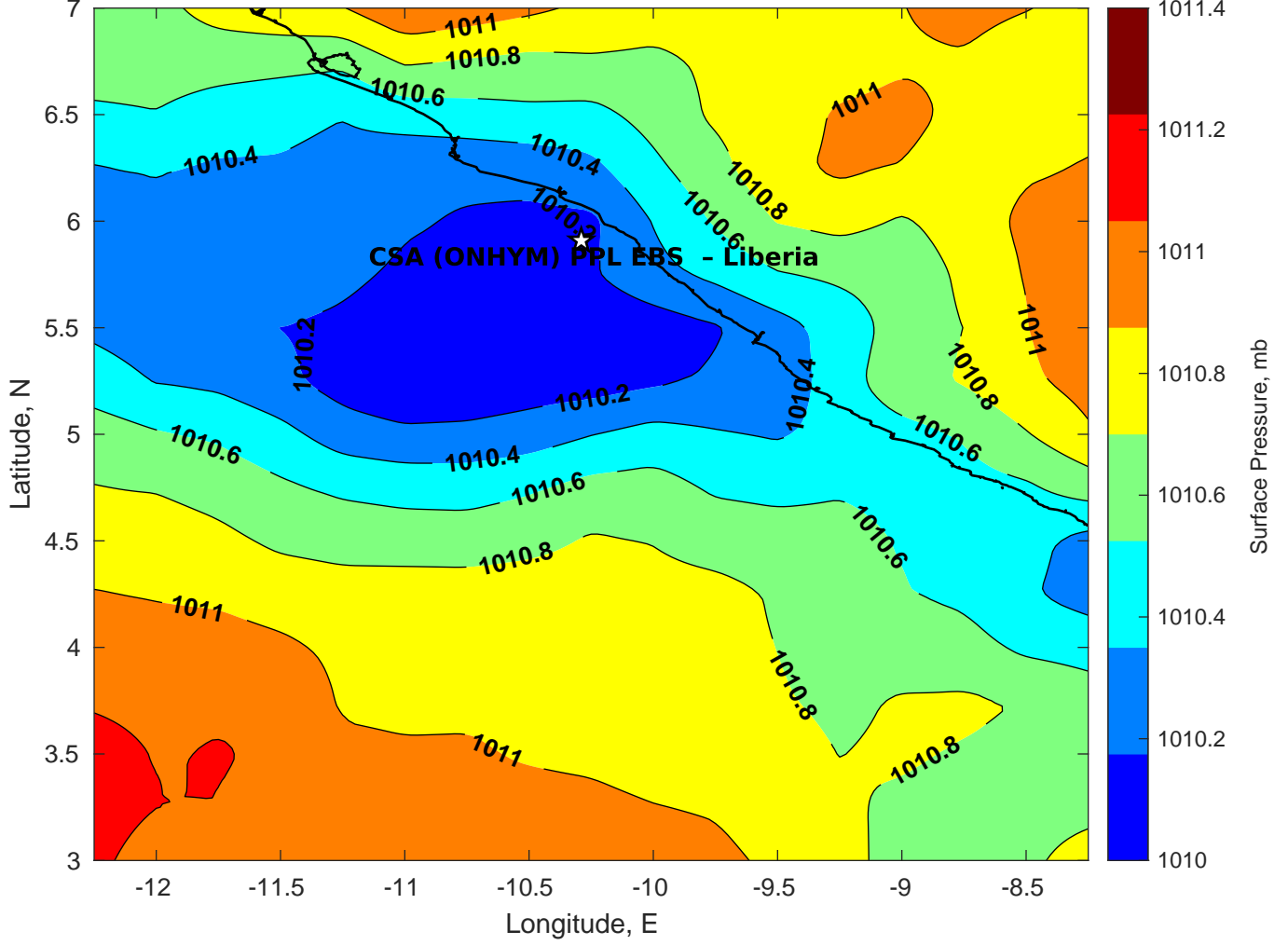
Surface Pressure (mb) for CSA (ONHYM) PPL EBS - Liberia at 17-Feb-2025 00:00:00
