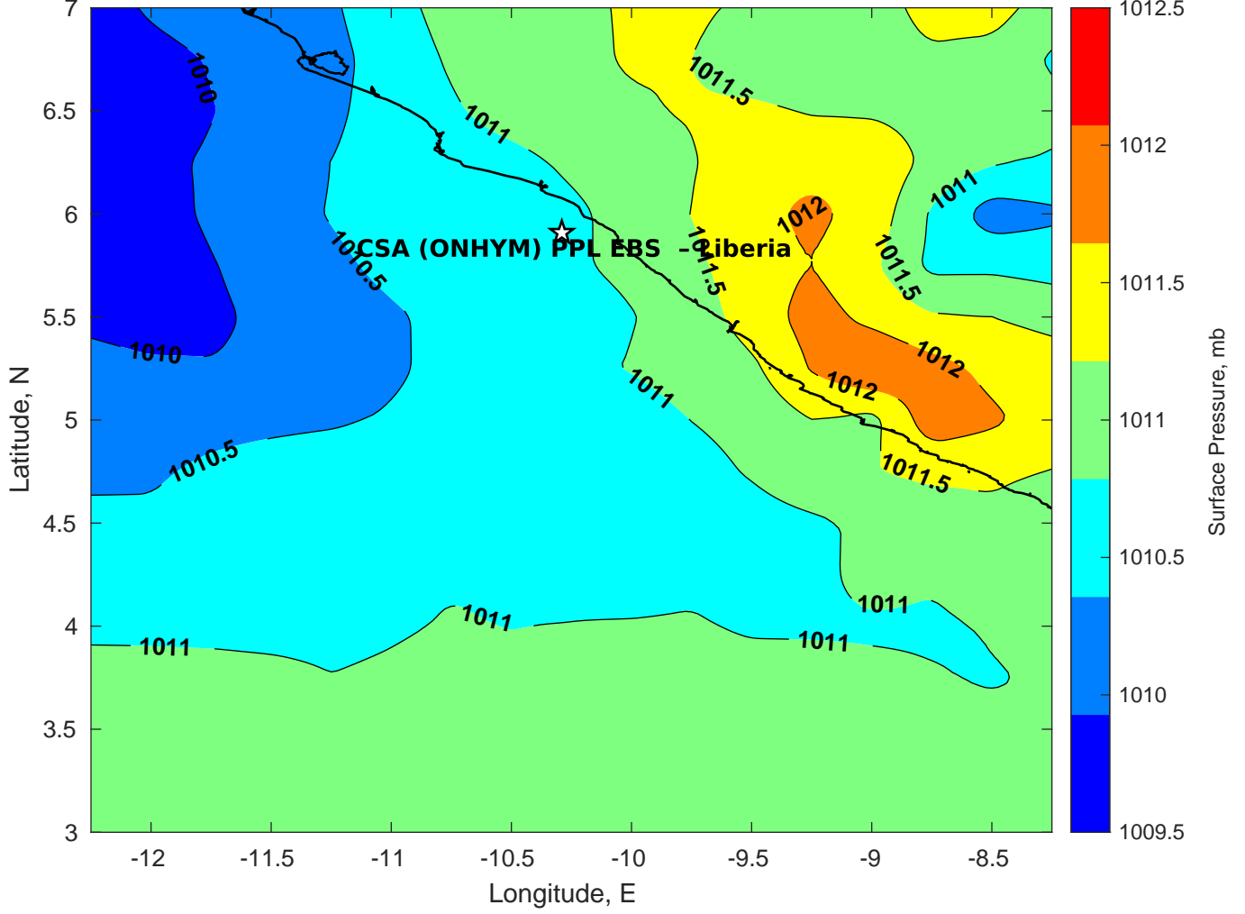
Surface Pressure (mb) for CSA (ONHYM) PPL EBS - Liberia at 19-Feb-2025 00:00:00
