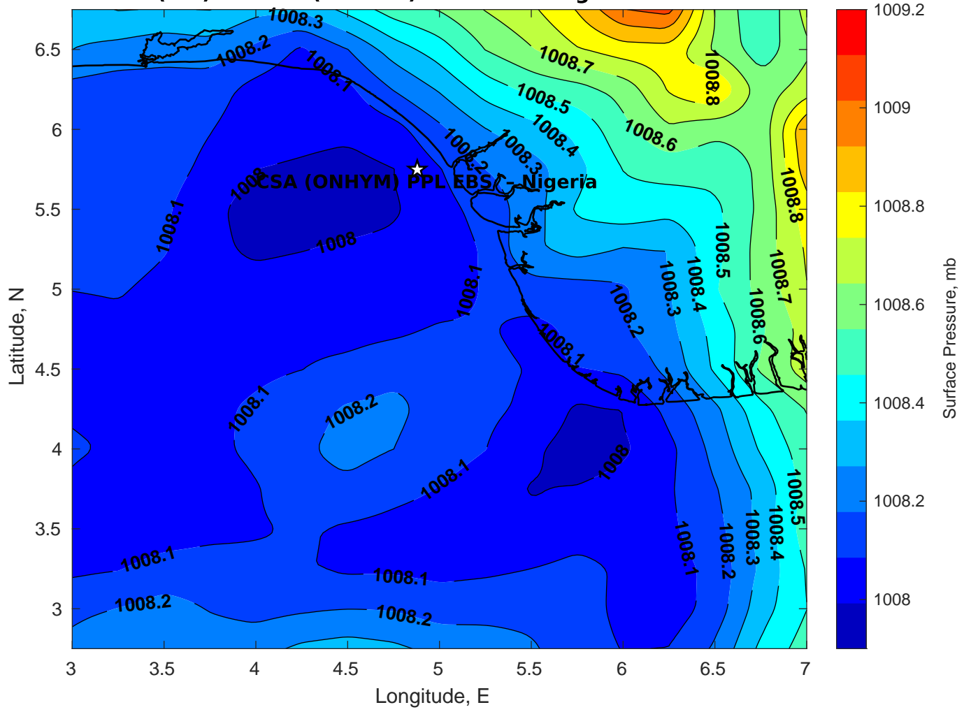
Surface Pressure (mb) for CSA (ONHYM) PPL EBS - Nigeria at 18-Feb-2025 06:00:00
