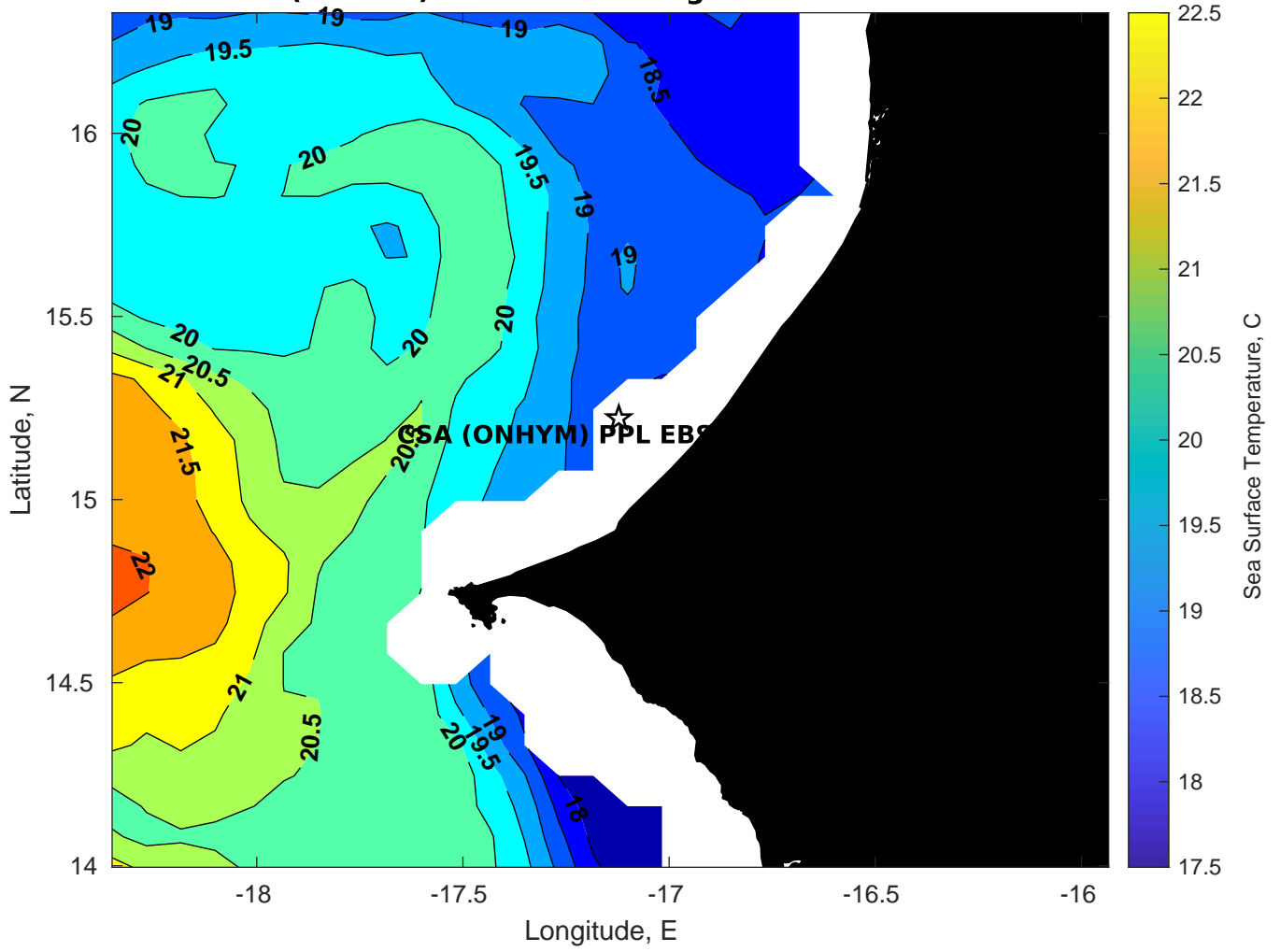
SST for CSA (ONHYM) PPL EBS - Senegal at 16-Feb-2025 00:00:00
