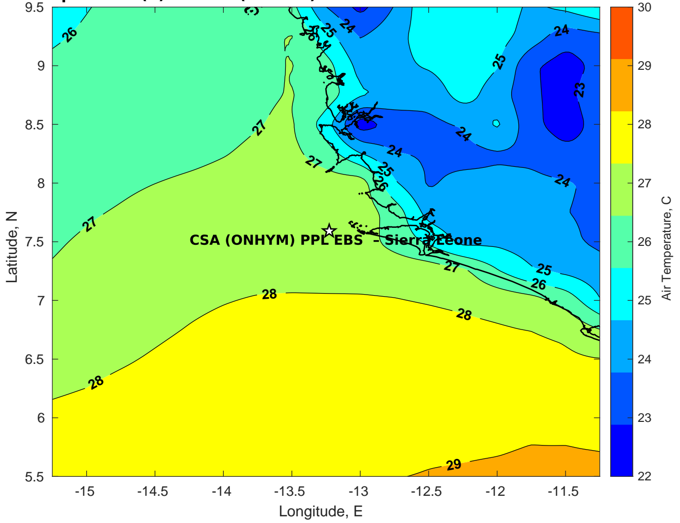
Air Temperature (C) for CSA (ONHYM) PPL EBS - Sierra Leone at 17-Feb-2025
