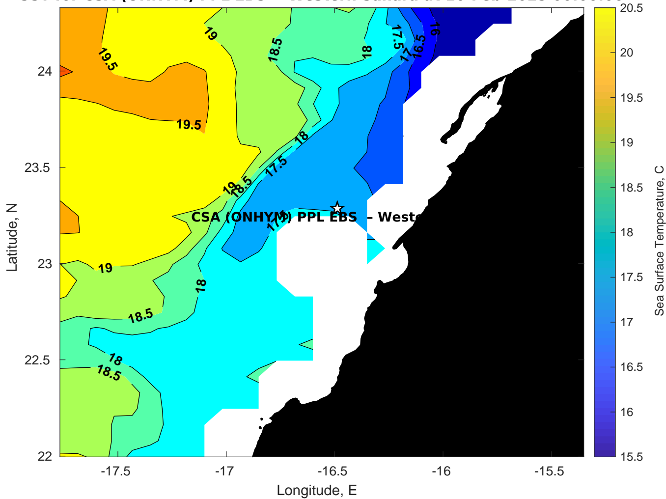
SST for CSA (ONHYM) PPL EBS - Western Sahara at 16-Feb-2025 00:00:00
