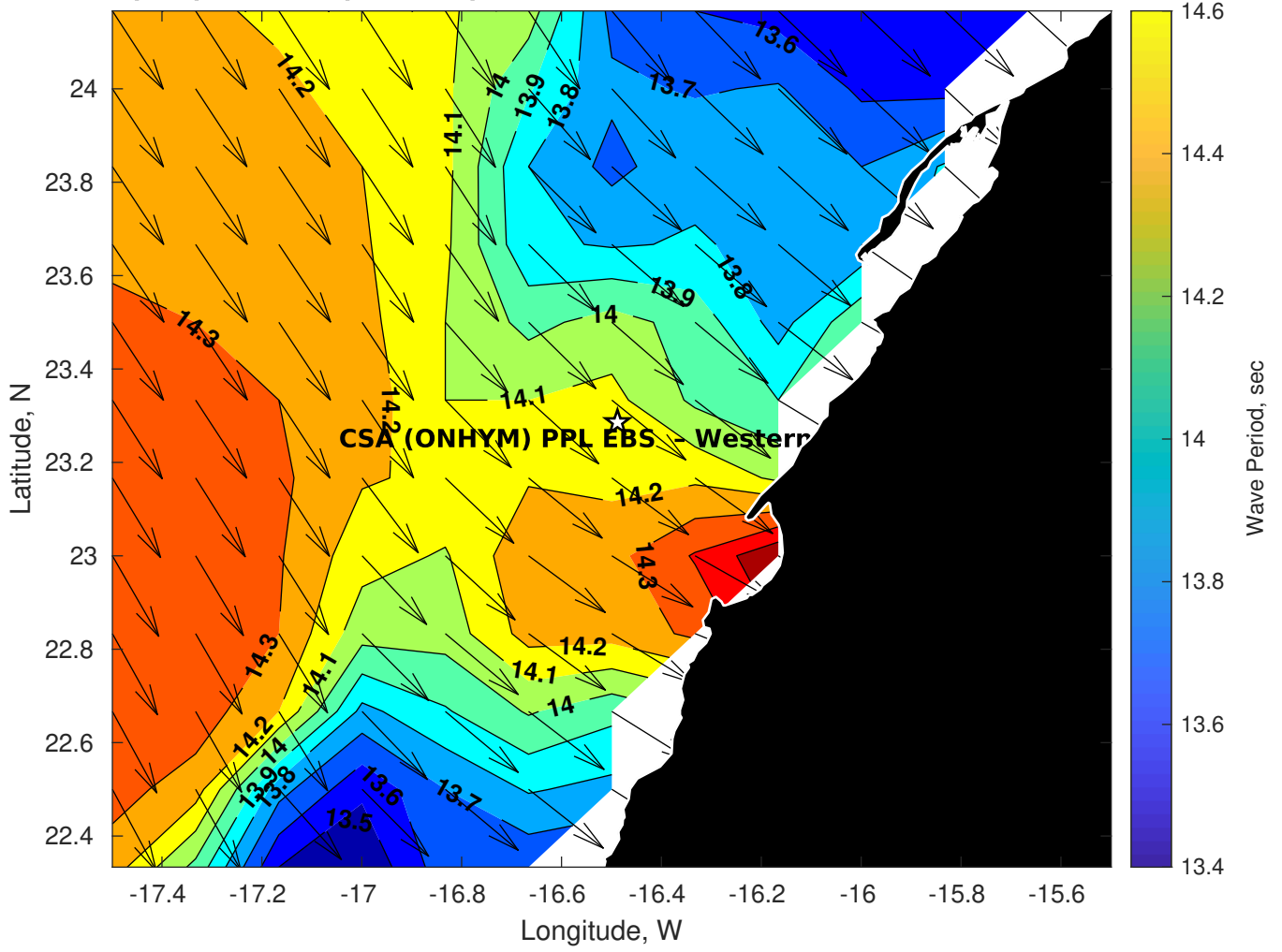
Wave Period (sec) for CSA (ONHYM) PPL EBS - Western Sahara at 17-Feb-2025 09:00:00
