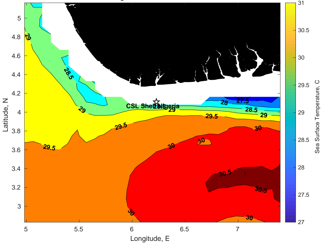
SST for CSL Shell Nigeria at 16-Feb-2025 00:00:00
