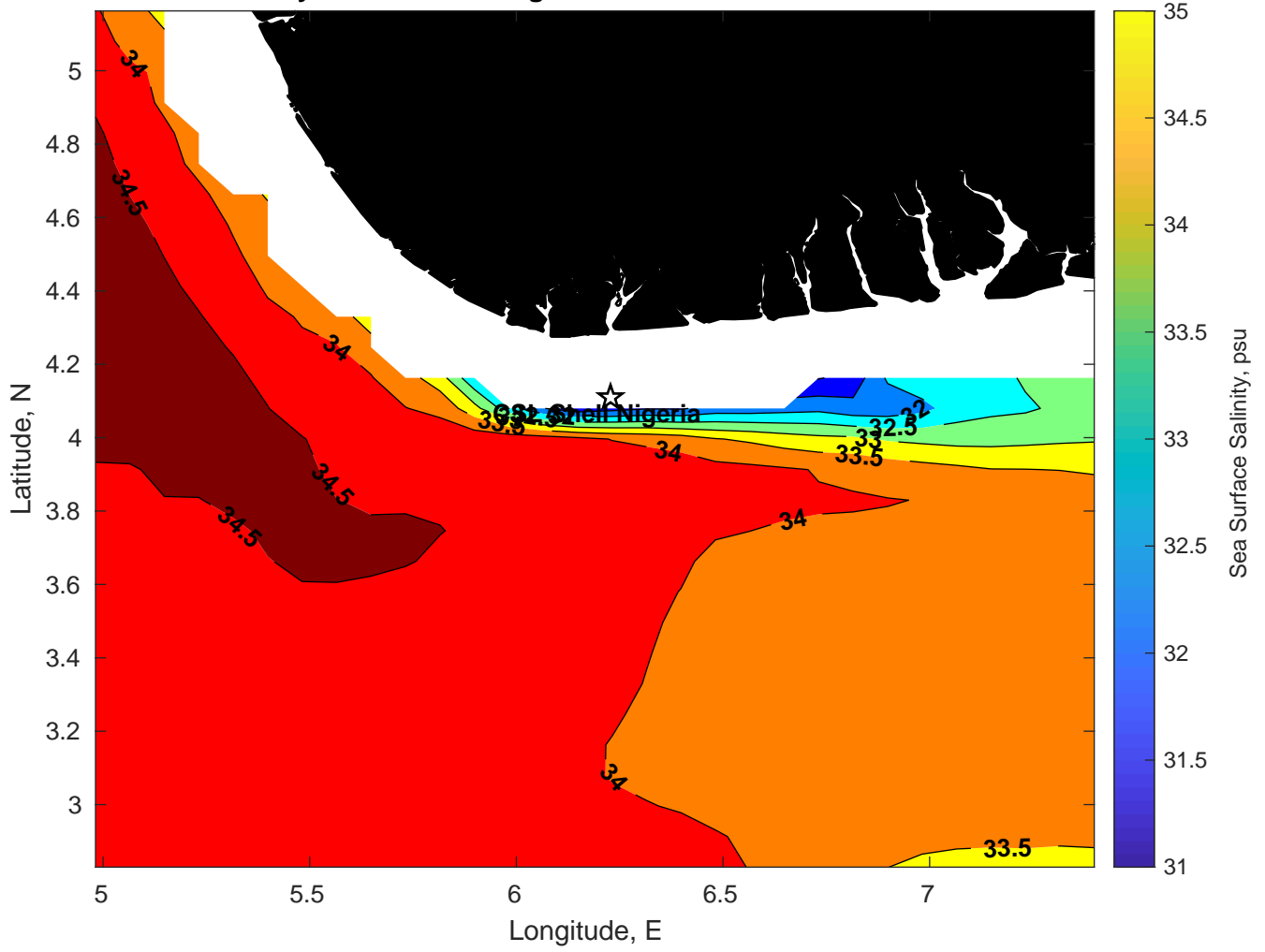
Surface Salinity for CSL Shell Nigeria at 16-Feb-2025 00:00:00
