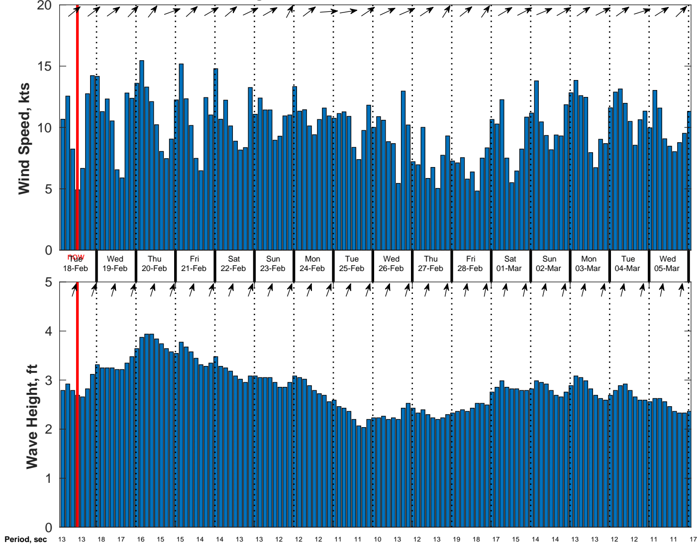
Wind & Wave Forecast for CSL Shell Nigeria from 17-Feb-2025 02:00:00 to 05-Mar-2025 02:00:00
