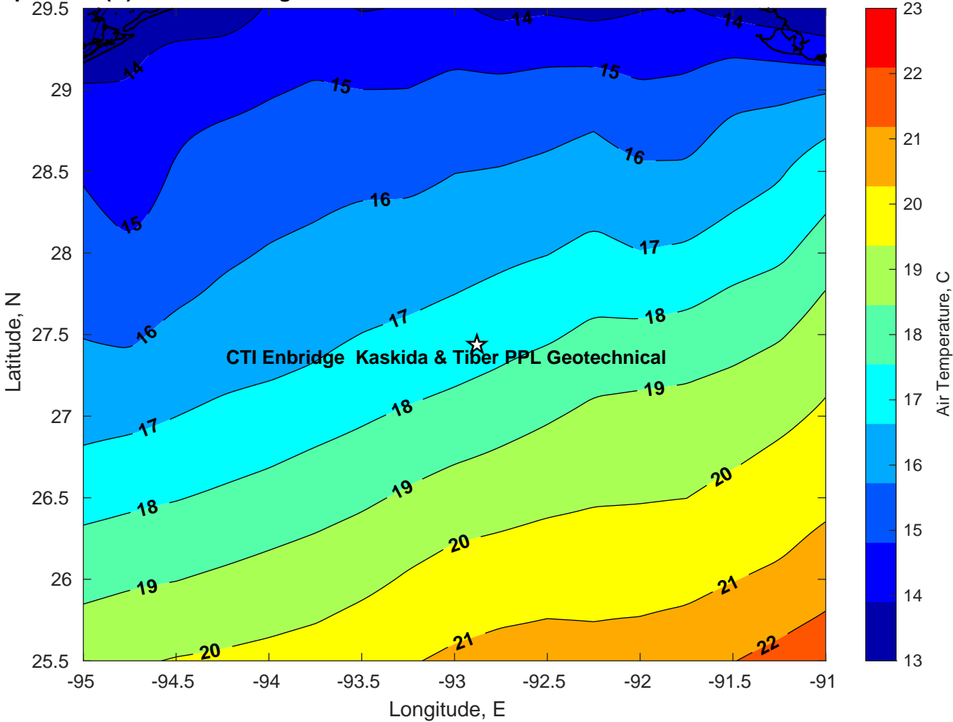
Air Temperature (C) for CTI Enbridge Kaskida & Tiber PPL Geotechnical at 17-Feb-2025
