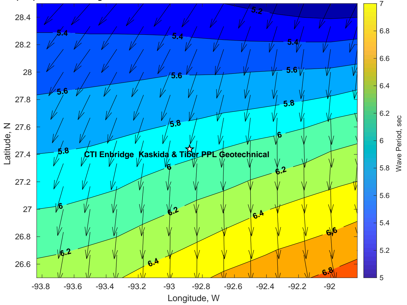
Wave Period (sec) for CTI Enbridge Kaskida & Tiber PPL Geotechnical at 17-Feb-2025 09:00:00
